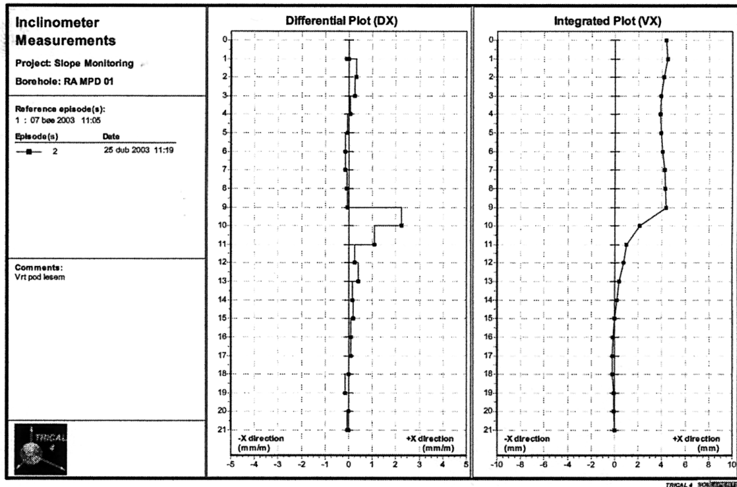
Figure 8: Unexpected inclinometer results showing a new plastic zone in deep location
