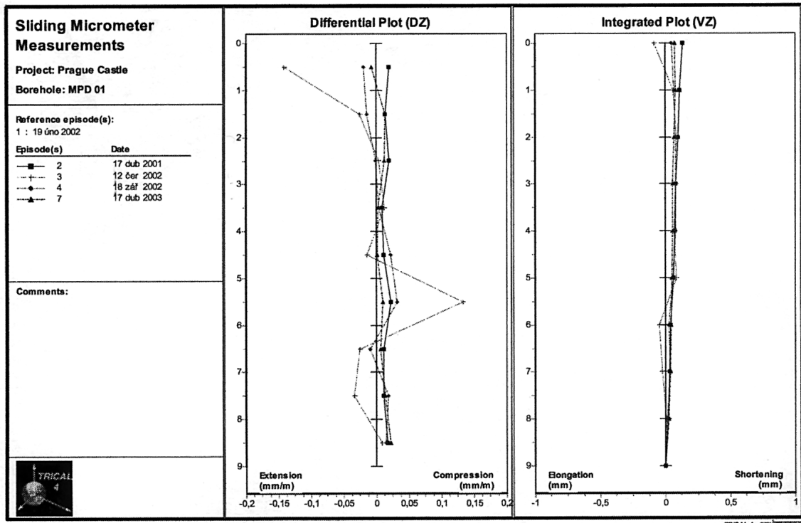
Figure 5: Axial deformation of footing and subsoil: differential and integrated
