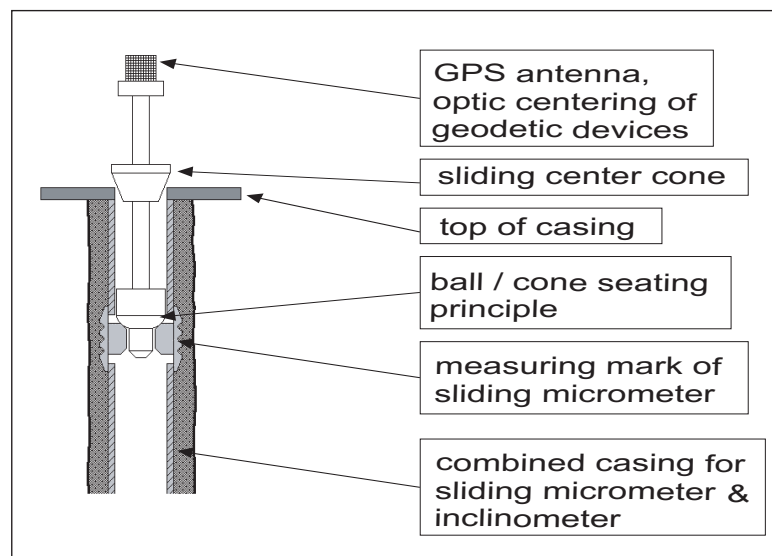
Figure 6: Insert tool to link high accuracy geotechnic and geodetic measurements
