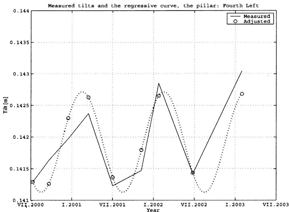
Figure 4: Horizontal shifts of pillar in section 4 left
