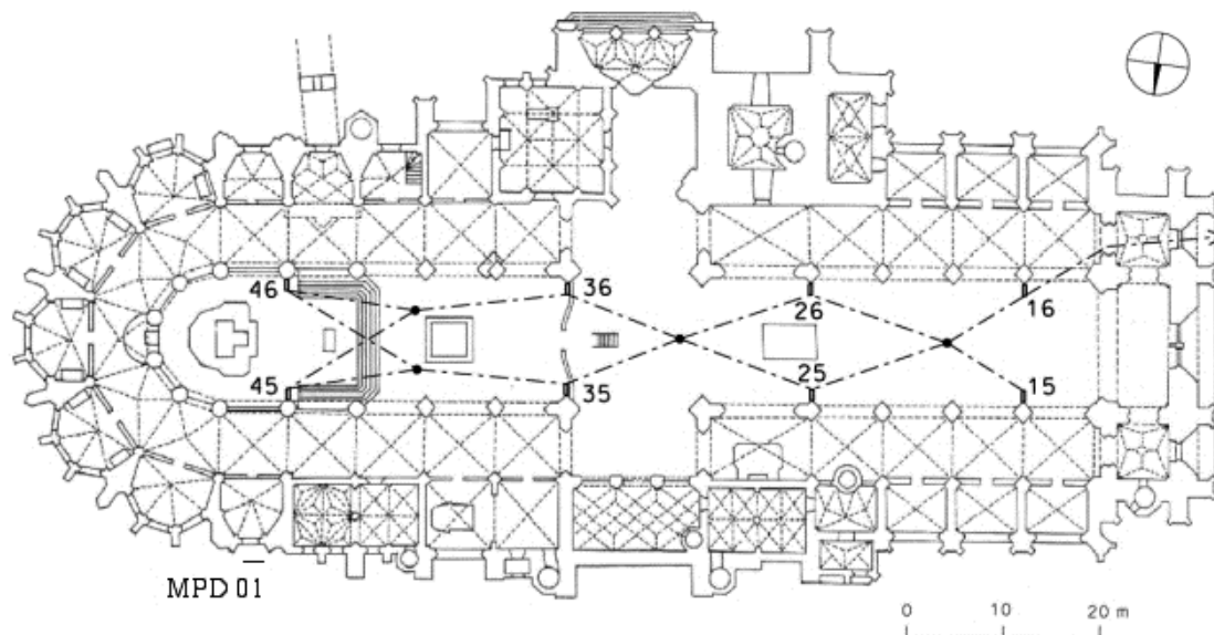
Figure 2: The scheme of benchmarks and locations of sections for trigonometric measurement and MPD 01 reference point at the cathedral
