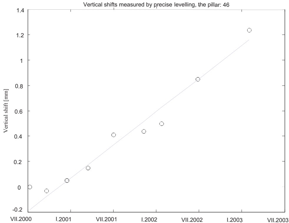
Figure 3: Estimation of annual vertical shift by regression analysis
