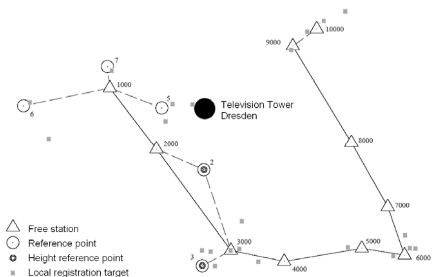
Figure 5: Network diagram
