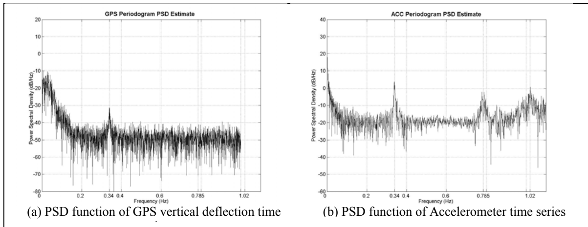
Figure 8: PSD functions of GPS and Accelerometer time series for station CENTRE
