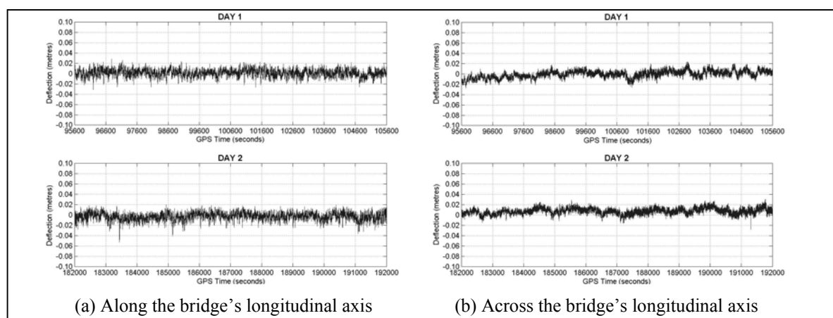
Figure 6: Horizontal deflections recorded at the bridge's tower
