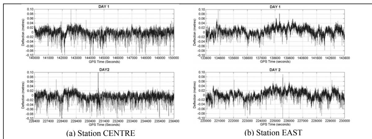
Figure 5: Vertical deflections recorded at the bridge's deck
