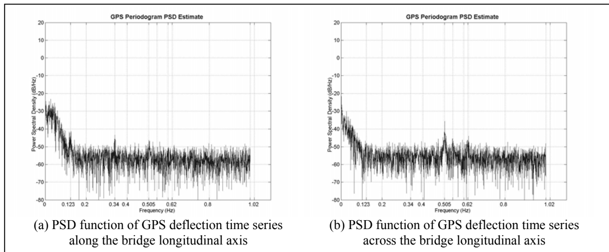
Figure 10: PSD functions of GPS time series for station TOWER
