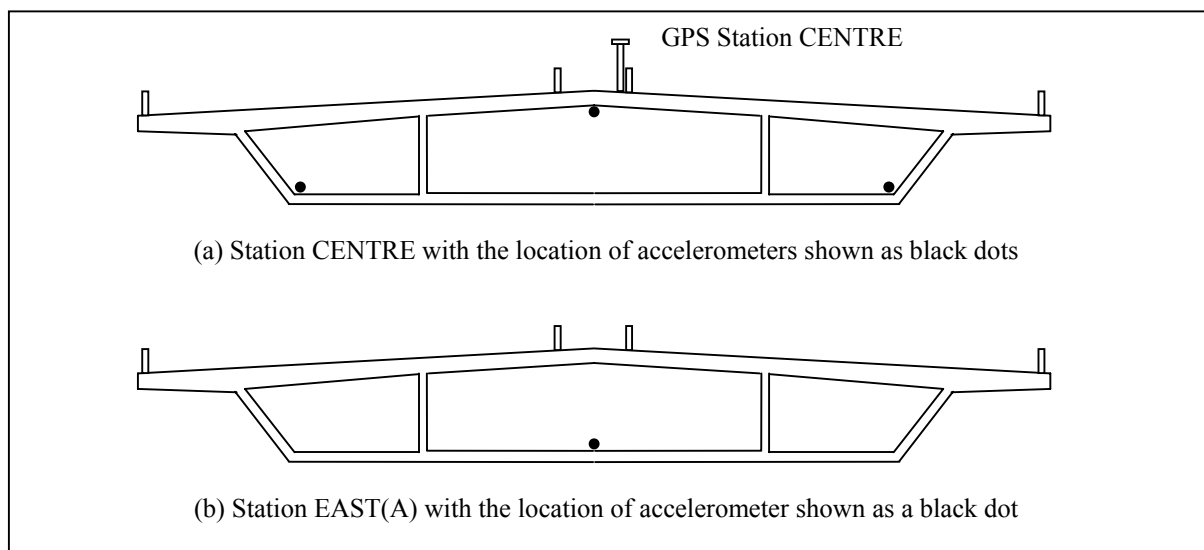
Figure 4: General layout of accelerometer installation for stations CENTRE and EAST(A)
