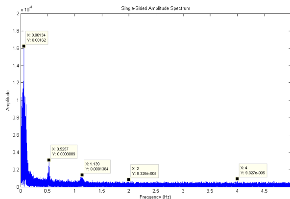
Figure 11 - Amplitude Spectrum for Midpoint 1 Vertical Deflection.
