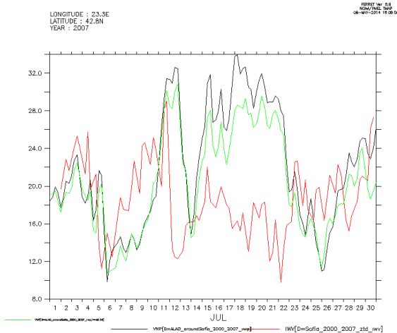
Figure 3b: Modelled (black and green lines) and observed (red line) IWV in July 2007.
