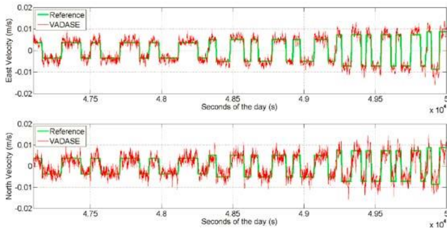
Figure 12 VADASE East and North estimated velocities compared to the reference solution during a sensitivity test.
