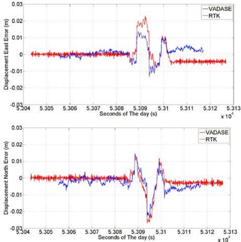
Figure 16 10 Hz VADASE vs RTK solution deviation in comparison to the reference movement for the 16 seconds diagonal movement scenario.
