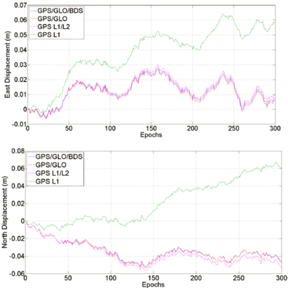
Figure 10 East and North displacements computed by integrating the velocities in Figure 9
