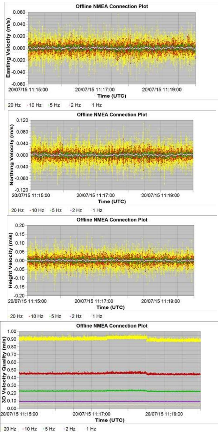
Figure 6 Comparison between different GNSS data rates solutions for East, North, and Height velocities of a static reference station in Heerbrugg.
