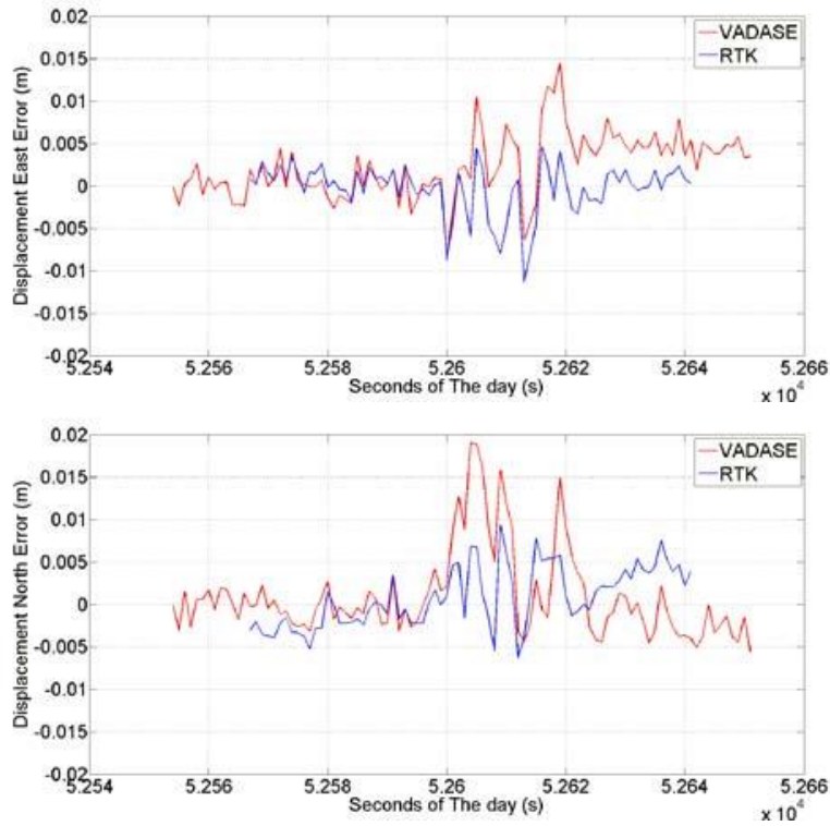
Figure 141 Hz VADASE vs RTK solution East & North deviations in comparison to the reference movement for the 25 seconds square movement scenario.
