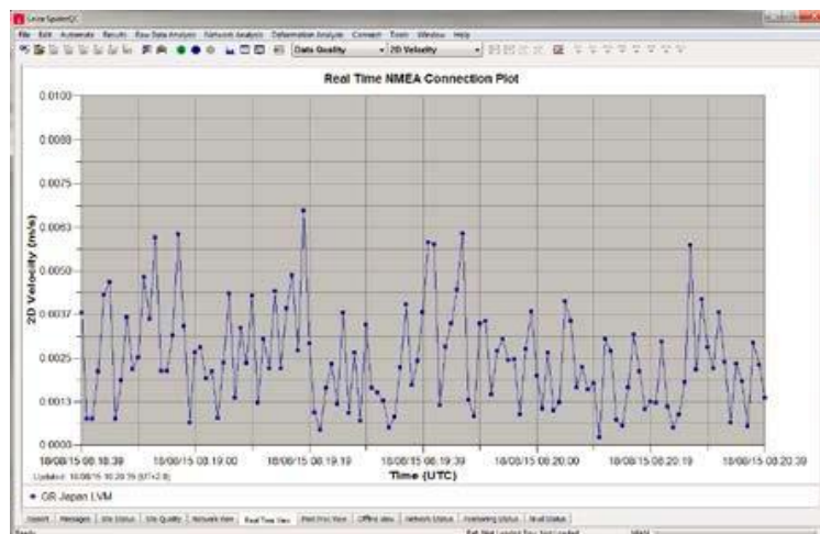
Figure 2 : Real-time NMEA plot of 2D-Velocity
