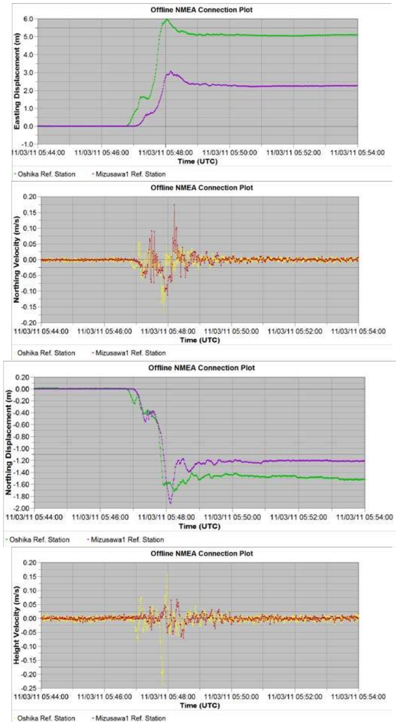
Figure 18 East, North, and Height velocities and displacements of Oshika and Mizusawa1 reference stations during the 2011 earthquake off the Pacific coast of Tōhoku, Japan computed by Leica VADASE.
