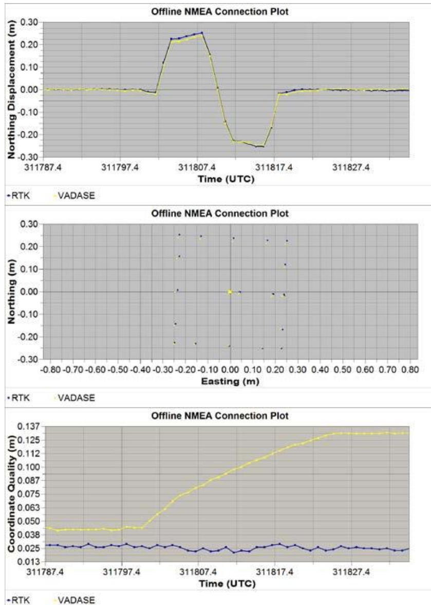
Figure 13 Above four graphs show 1 Hz VADASE vs RTK solution for the square movement scenario.
