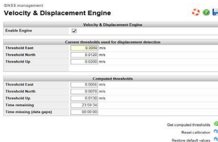
Figure 1 V&DE configuration page
