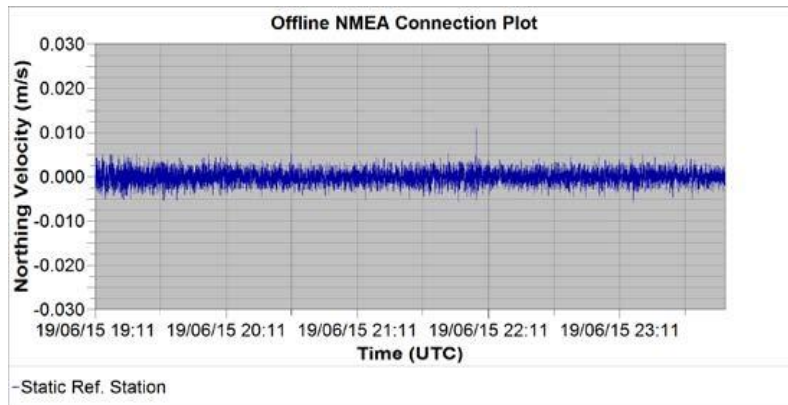
Figure 4 Northing velocity estimation by VADASE for a static reference station.
