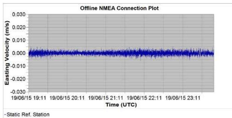
Figure 3 Easting velocity estimation by VADASE for a static reference station.
