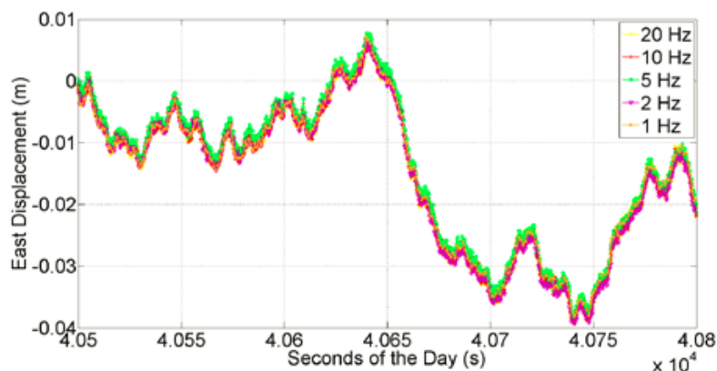
Figure 8 Comparison between different GNSS data rates solutions for east total displacement of a static GNSS reference station in Heerbrugg.
