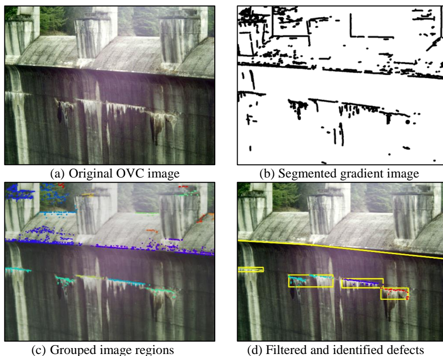
Figure 8: Important steps of the defect detection algorithm
