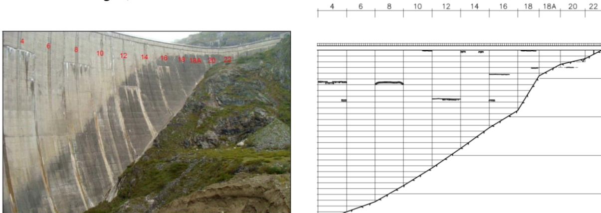
Figure 1: Photograph of the downstream side of the Drossen dam (left), corresponding CAD drawing showing defect locations (right, Verbund, 2011)
