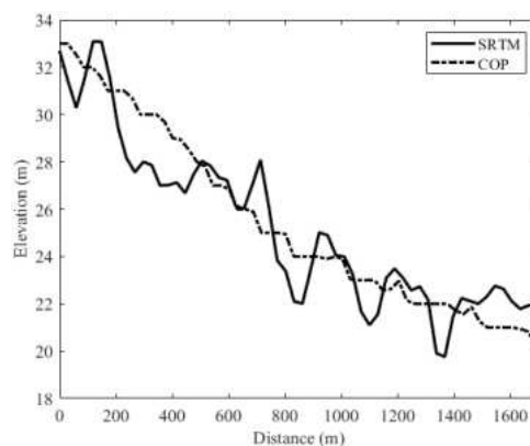
Figure 5. Profiles of the Grafton airport runway derived from the SRTM and COP models.
